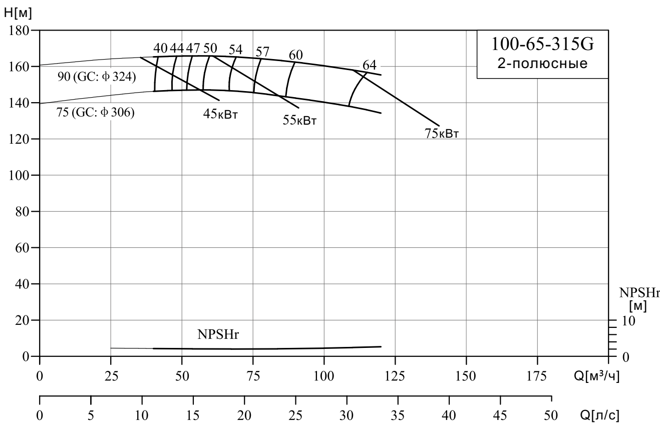
NIS100-65-315G/100-80-160G
