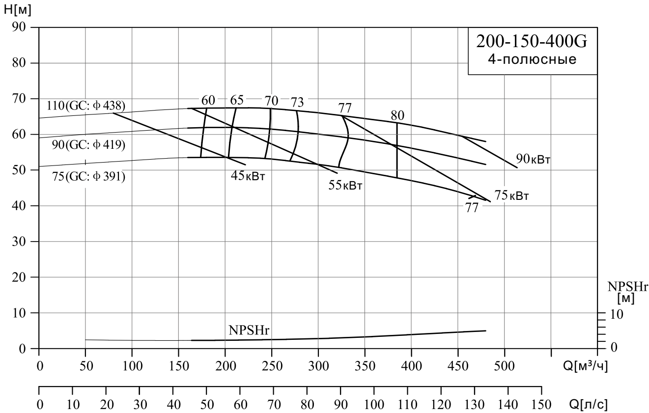
NIS200-150-400G
