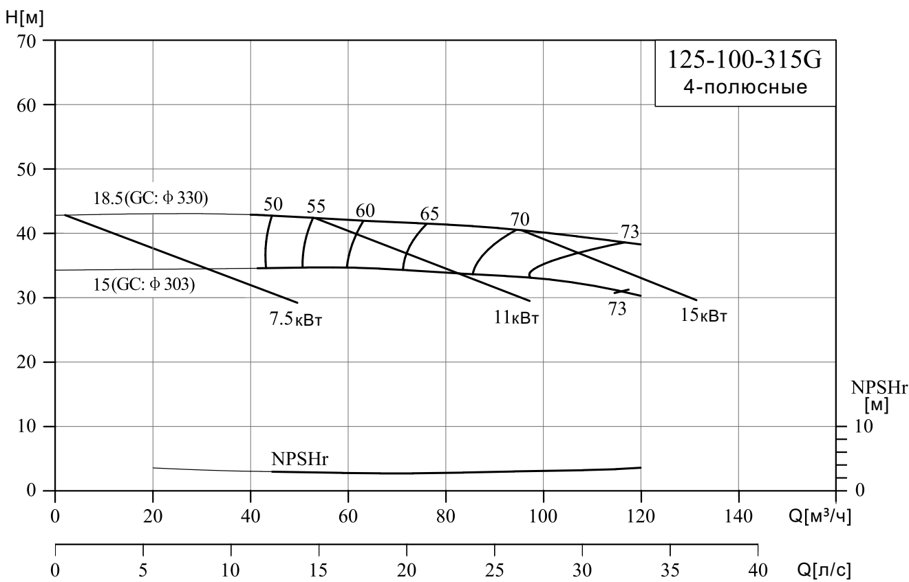
NIS125-100-315G/125-100-400G
