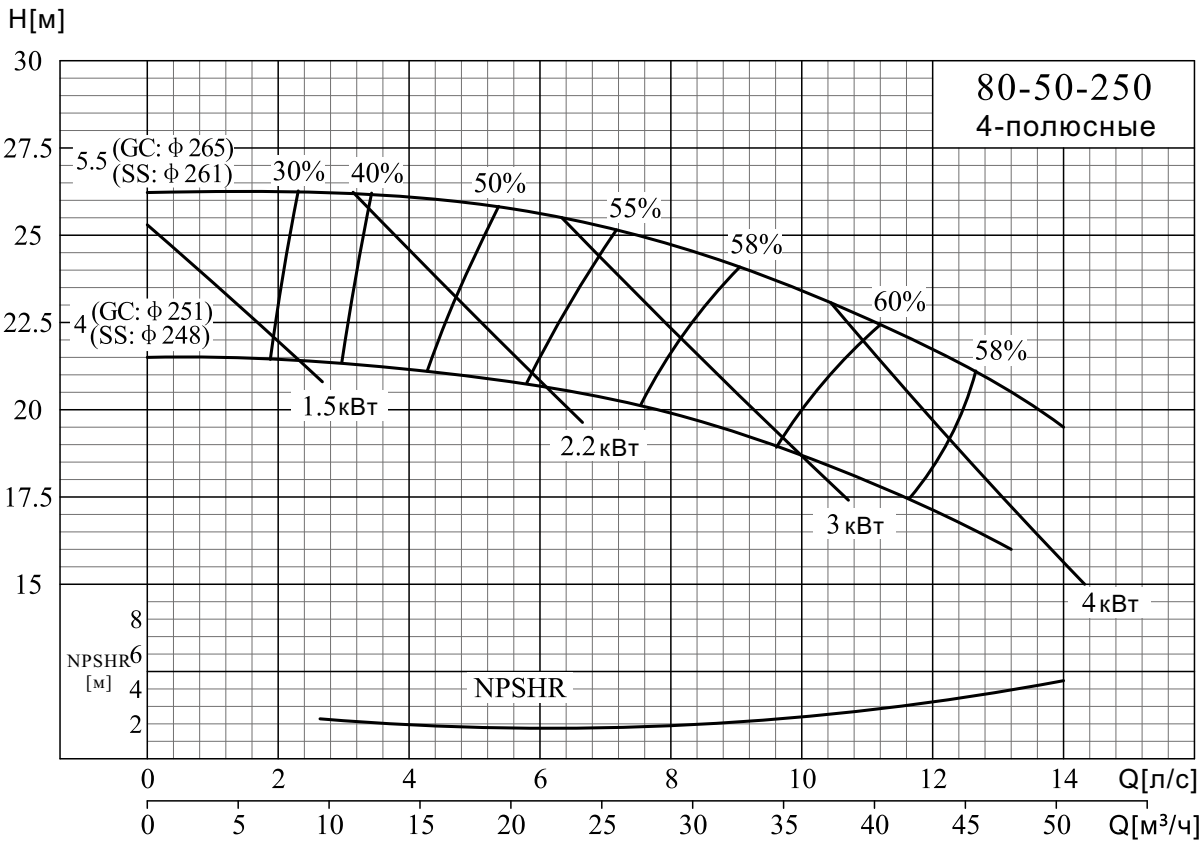
NISO,NIS,NISF 80-50-250/80-50-315
