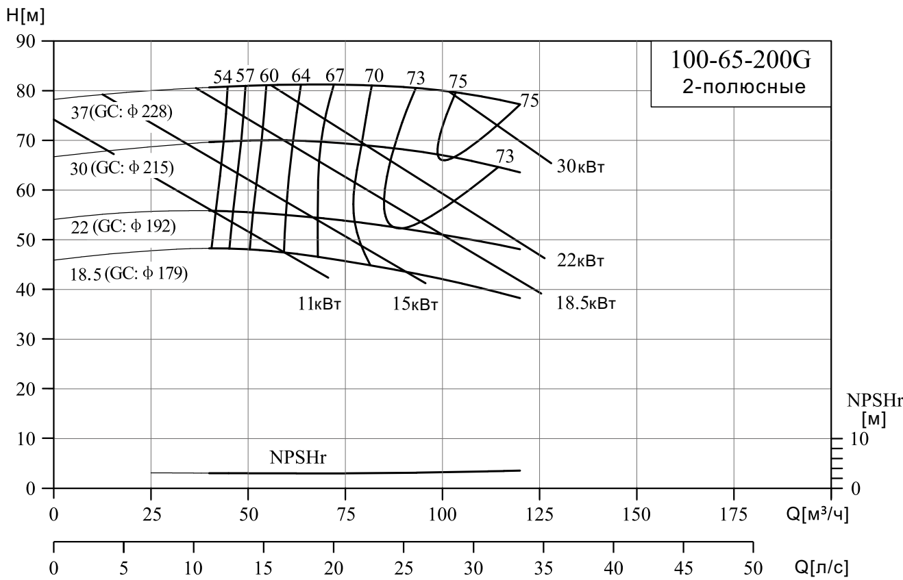
NIS100-65-200G/100-65-250G
