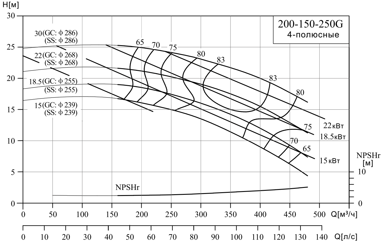
NIS200-150-250G/200-150-315G
